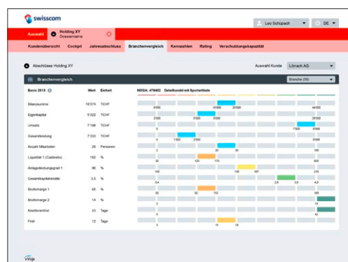
Application web
